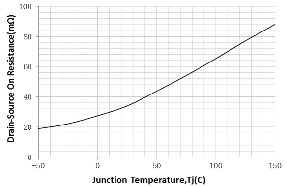
On-Resistance Variation vs. Temperature
